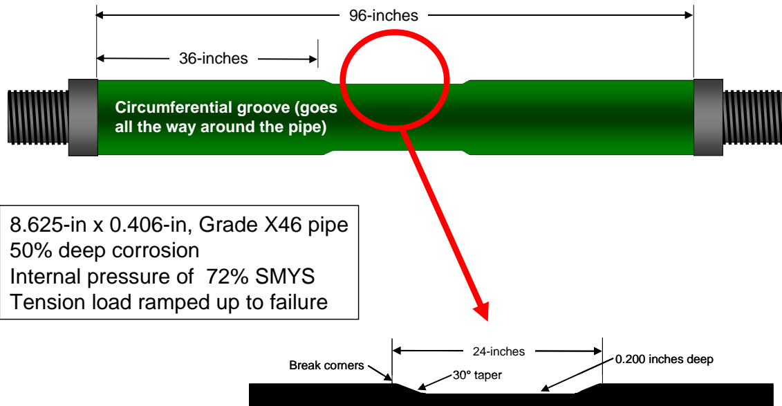
Figure 16 – Axial tension sample from prior MMS study
