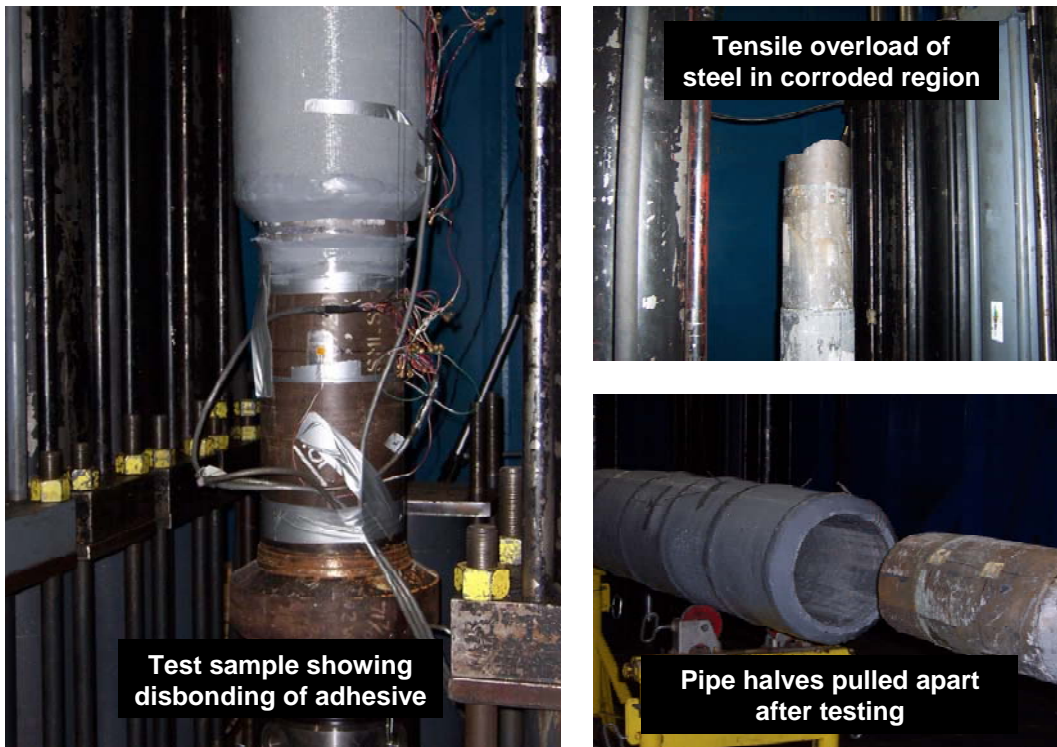
Tension Test Sample (failure in corroded region of repair)
