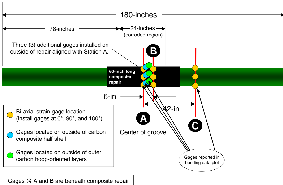
Figure 11 - Locations for strain gages of interest on CRA system samples
