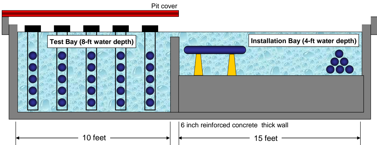
Figure 17 – Proposed saltwater test facility for 10,000 hour long-term study
