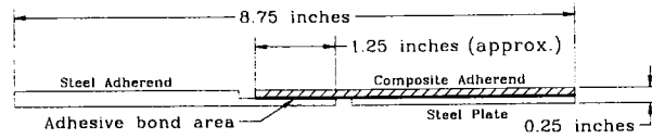
Composite on Steel Lap Shear Sample
