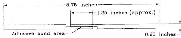
Steel on Steel Lap Shear Sample
